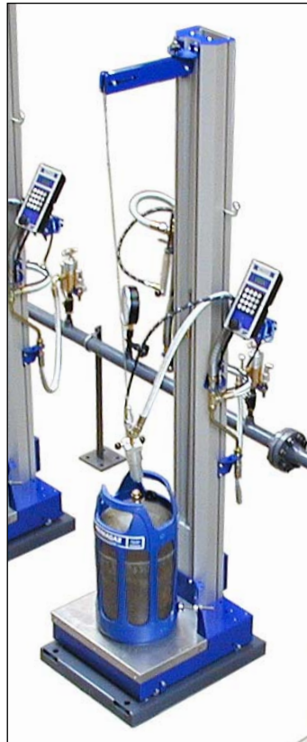
UFM universal filling machine
